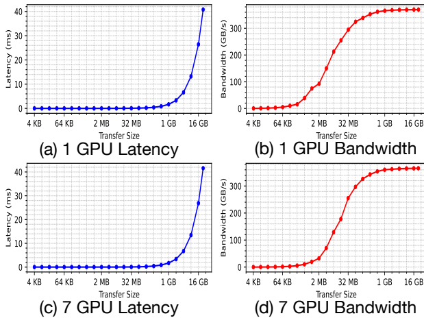
Fig. 6. Average latency (a, c) and bandwidth (b, d) for NCCL Broadcast with 1 and 7 receiver GPUs in NVLink 4.0
