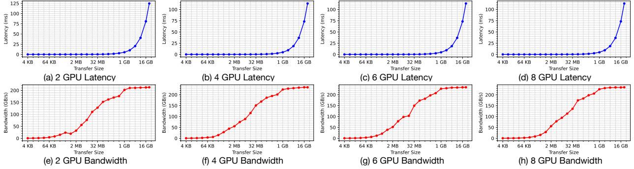
Fig. 3. Average latency (a–d) and per GPU bandwidth (e–h) for NCCL AllReduce with 2, 4, 6, 8 receiver GPUs
