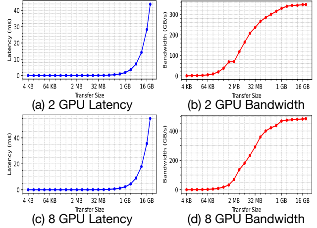
Fig. 7. Average latency (a, c) and bandwidth (b, d) for NCCL Allreduce with 2 and 8 receiver GPUs in NVLink 4.0
