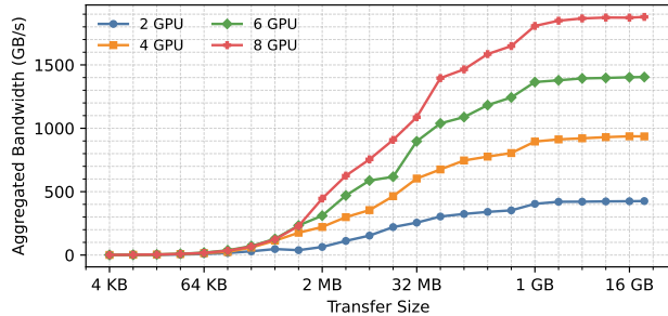
Fig. 4. The aggregated bandwidth of 2, 4, 6, 8 GPUs using NCCL AllReduce
