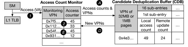
Fig. 16. Design and workflow of access count monitor
