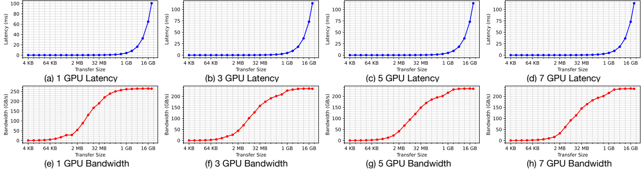
Fig. 2. Average latency (a–d) and bandwidth (e–h) for NCCL Broadcast with 1, 3, 5, and 7 receiver GPUs
