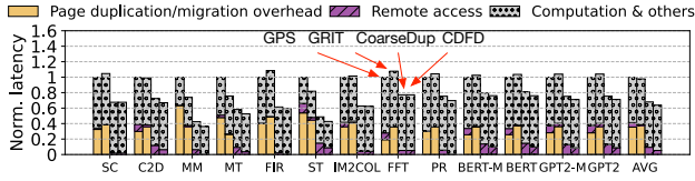
Fig. 18. Performance breakdown normalized to GPS
