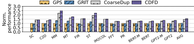
Fig. 24. End-to-end performance results under NVLink 4.0 Setting
