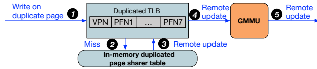
Fig. 13. Workflow of remote update
