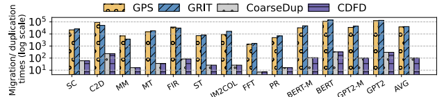
Fig. 21. Migration / Duplication times in log scale
