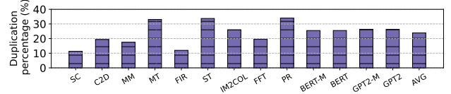
Fig. 20. Average duplication percentage relative to memory footprint
