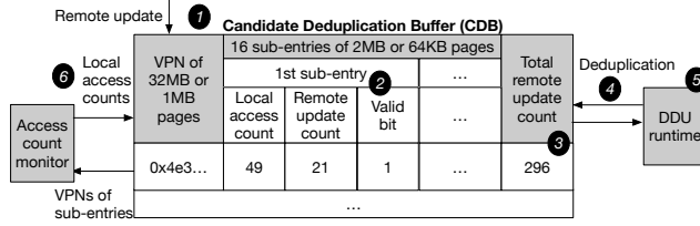
Fig. 15. Design and workflow of CDB
