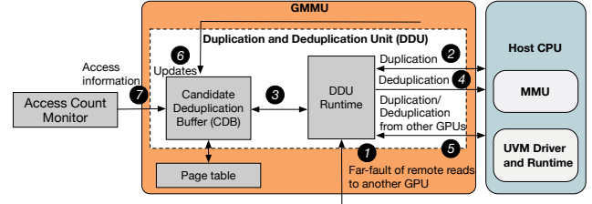
Fig. 14. Workflow of duplication and deduplication unit
