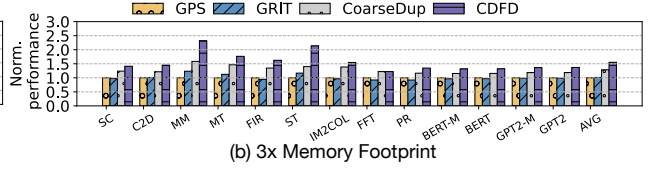
Fig. 22. End-to-end performance results relative to GPS under (a) 2.5\times memory footprint (b) 3.0\times memory footprint
