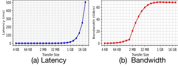
Fig. 5. Average latency (a) and bandwidth (b) results under UVM using cudaMemPrefetchAsync() between two GPUs interconnected via NVLink 3.0
