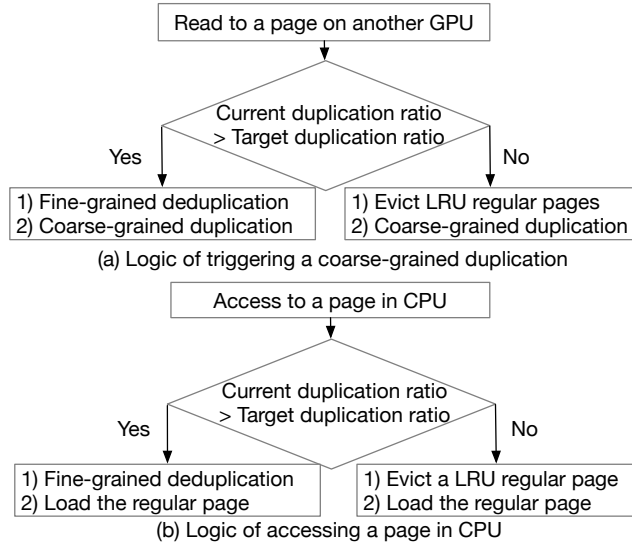
Fig. 11. Logic for handling a read to another GPU (a) or an access to a page in CPU (b) when local GPU memory is full
