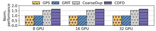
Fig. 23. Average performance with 8, 16, and 32 GPUs relative to GPS
