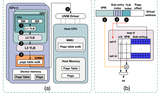
Fig. 1. UVM-managed Multi-GPU overview
